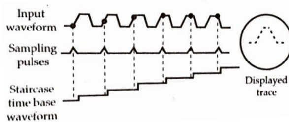
Fig: Sampling Principle and Display of dots
