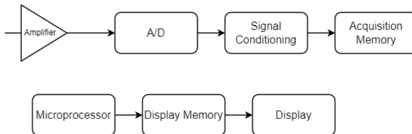
Fig: Block Diagram of Oscilloscope
